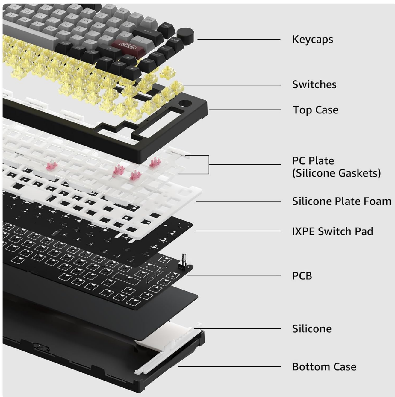
Figure 15: Internal structure of the Akko 5075B Plus keyboard, showing various layers for optimized noise reduction and typing feel.
