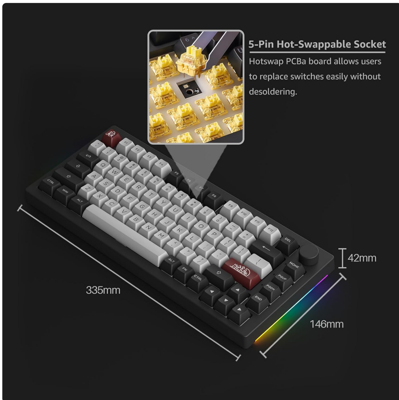
Figure 10: Hot-swappable PCB allowing users to easily replace switches.
