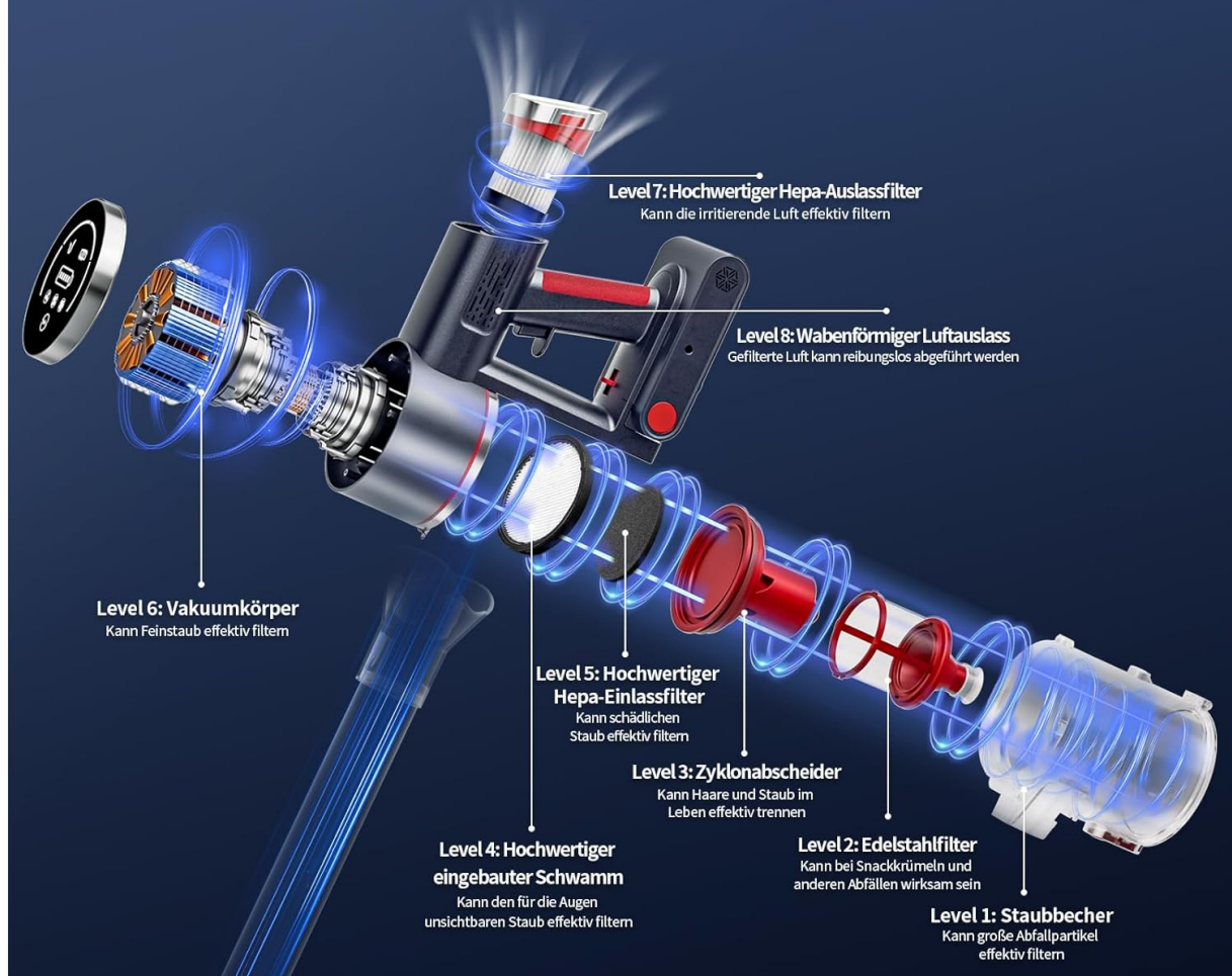
Image 5.1: Exploded view of the 8-stage high-efficiency filtration system.
