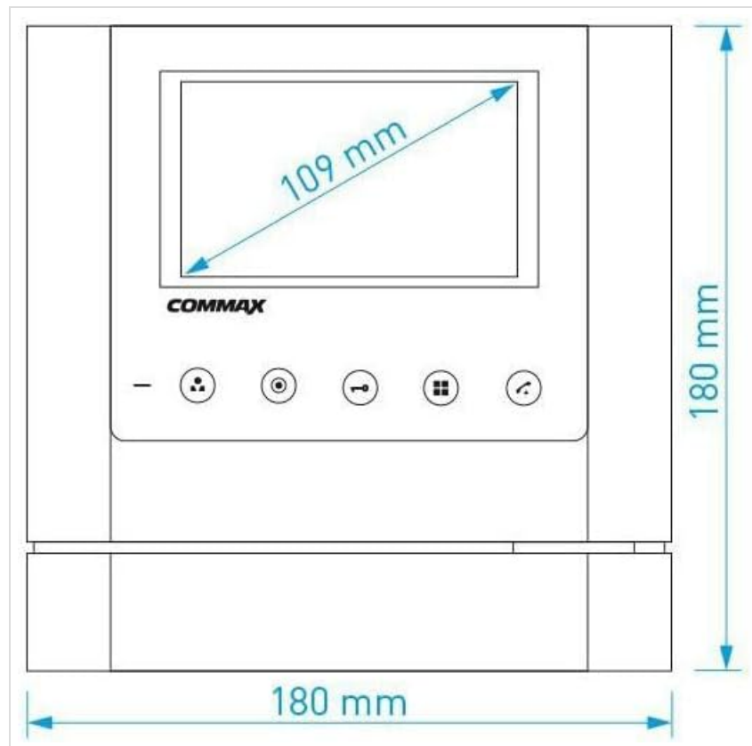
Figure 3.1: Technical drawing illustrating the dimensions of the COMMAX CDV-43M monitor. The diagram shows a width of 180 mm and a height of 180 mm, with the 4.3-inch LCD screen measuring 109 mm diagonally.
