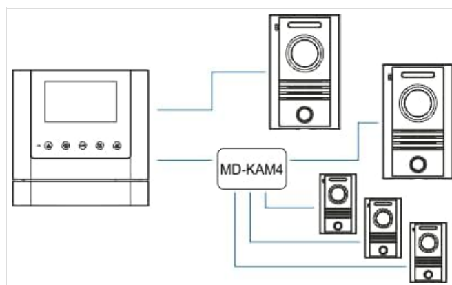
Figure 3.2: Schematic diagram demonstrating the connection of the COMMAX CDV-43M monitor to multiple door cameras and interphones via an MD-KAM4 distributor. This illustrates a typical multi-unit installation setup.
