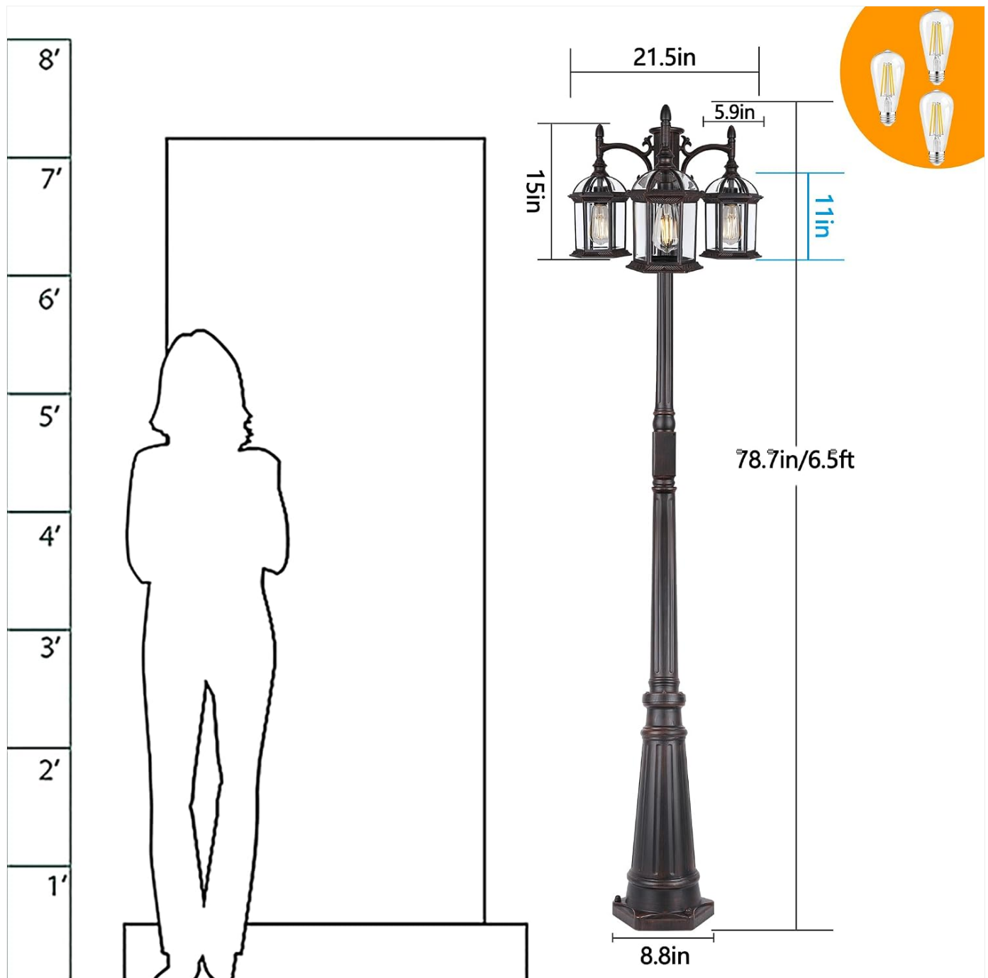
Figure 4: Product dimensions for installation planning. The lamp post is approximately 6.5 feet tall.
