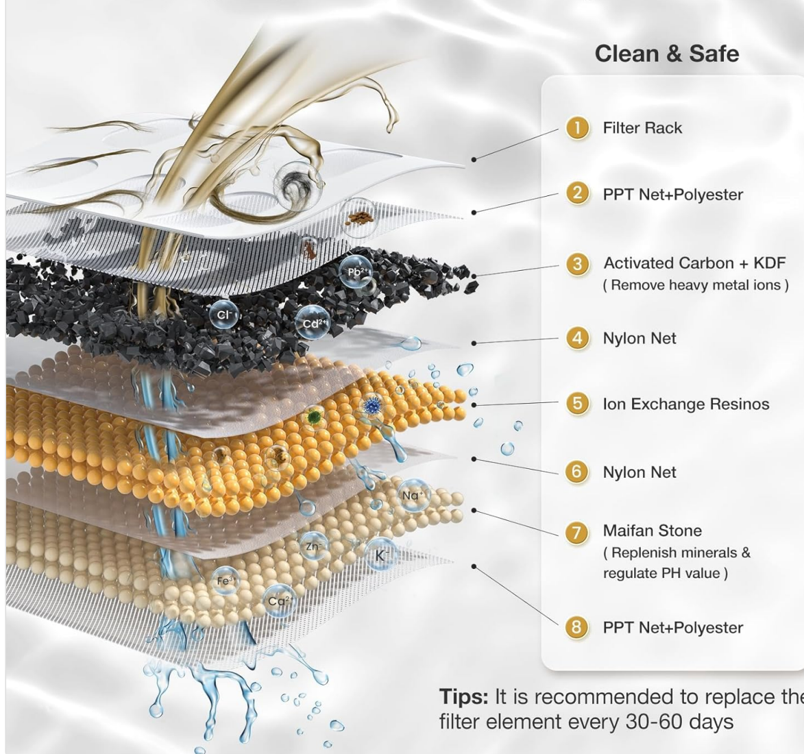
Image 5.2: PETGUGU PF1 8-Layer Filtration Design. This detailed diagram illustrates the eight layers of the filtration system, including activated carbon, ion exchange resin, and KDF materials, highlighting their function in purifying water.
