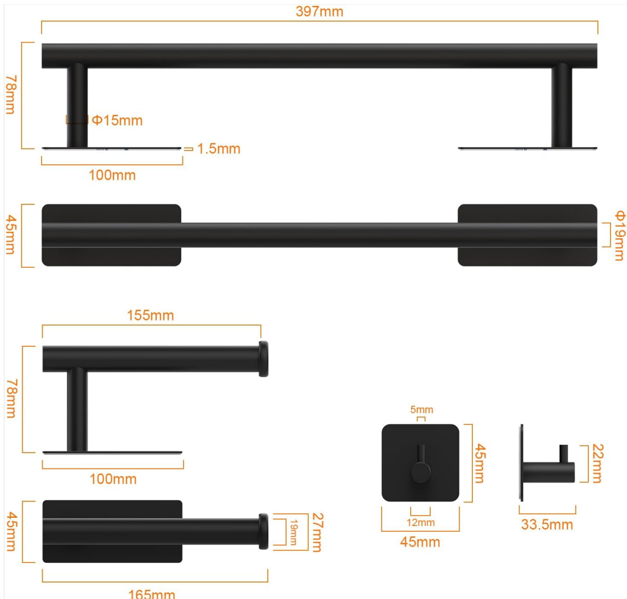
Image: Technical drawing showing the precise dimensions of each accessory in the set.
