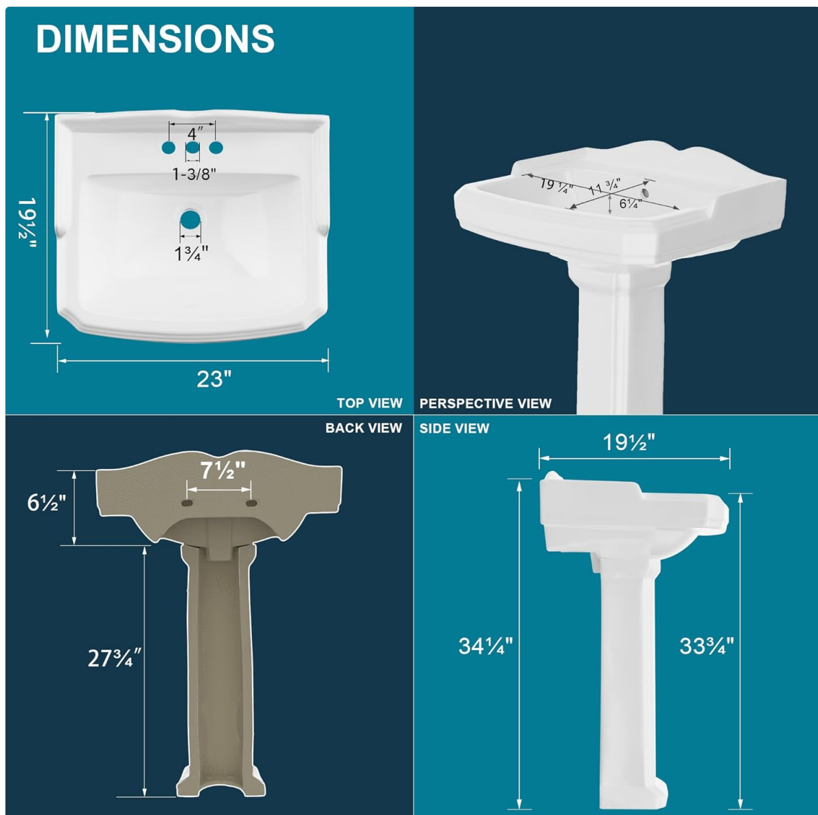
Image 3.1: Detailed dimensions of the sink basin and pedestal from various views.
