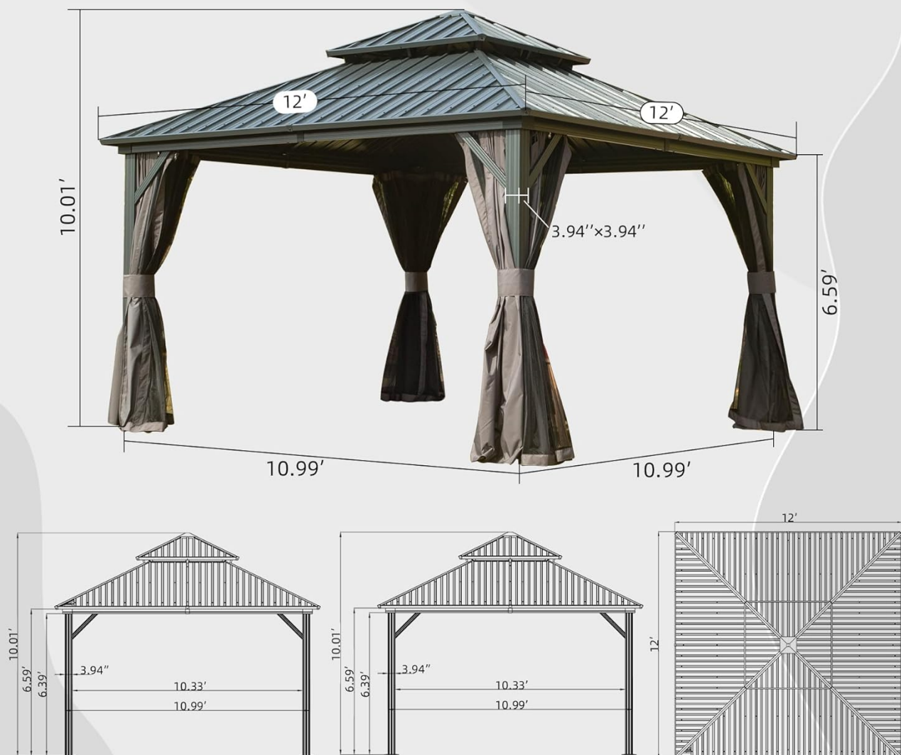
Image 3: Dimensional drawing of the Domi 12x12FT Gazebo.
