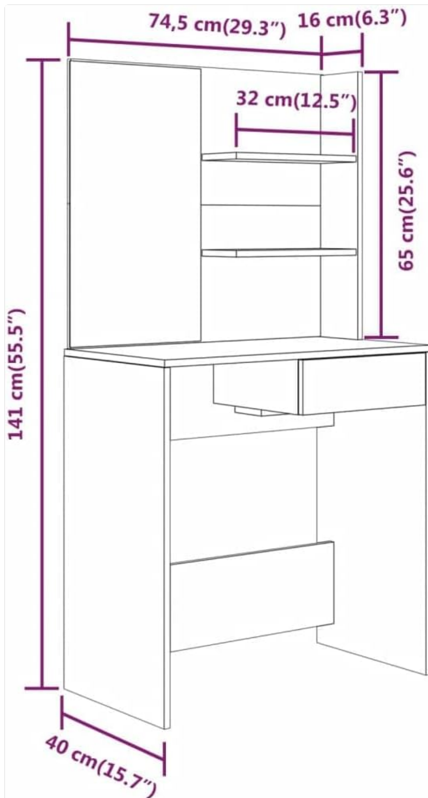
Figure 7: Detailed dimensions of the dressing table.
