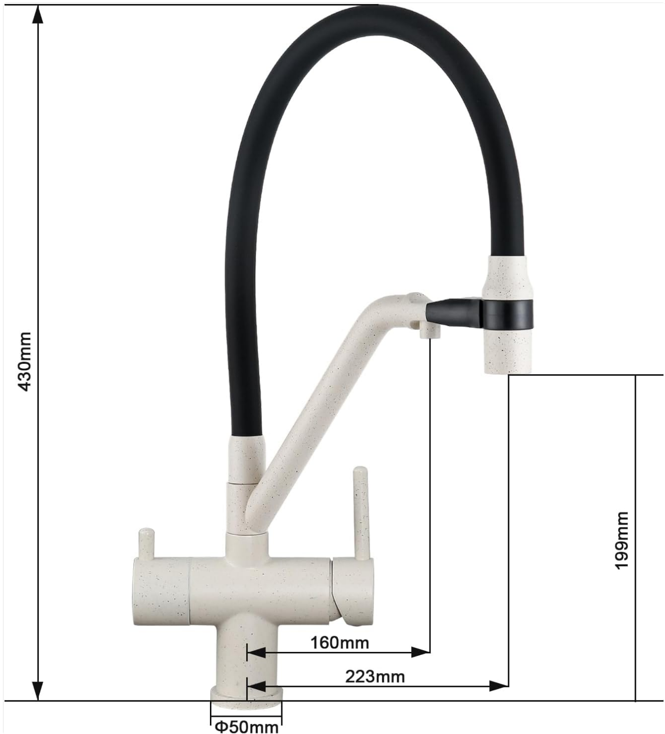
Figure 2.1: Faucet Dimensions (in millimeters)
