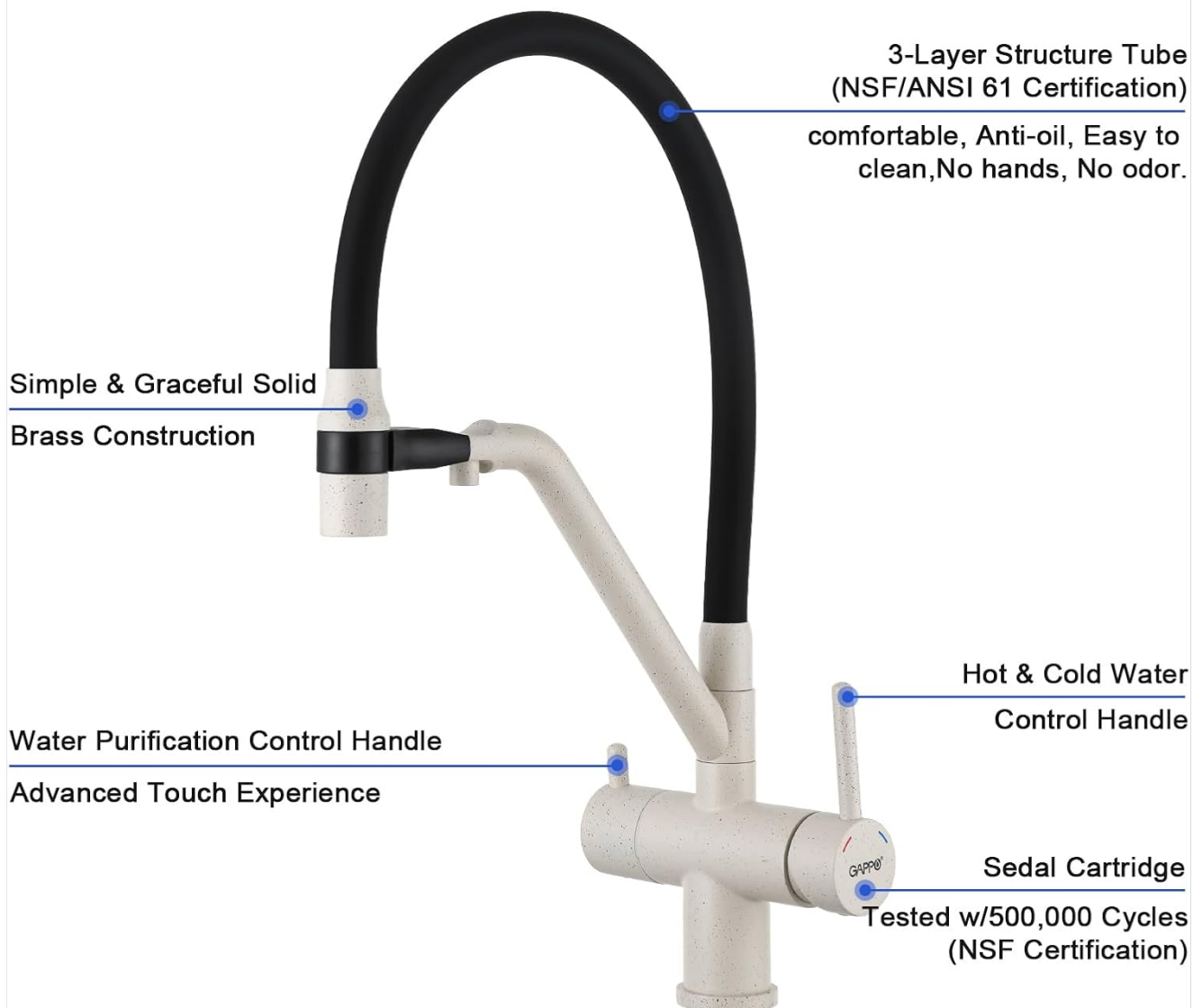
Figure 1.2: Labeled components of the GAPPO Kitchen Faucet
