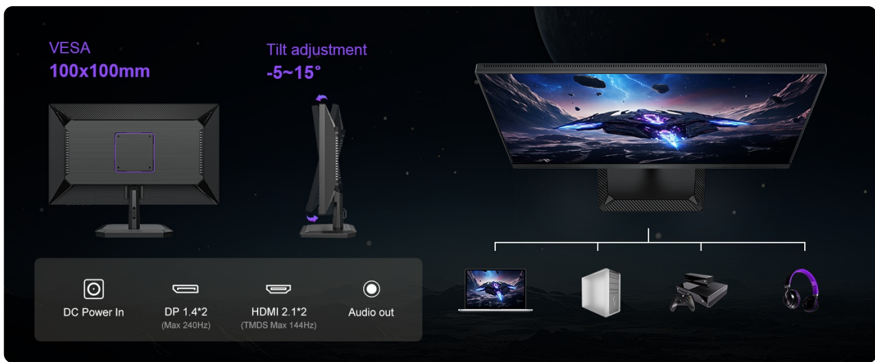
Image: The monitor highlighting its VESA mount (100x100mm) and tilt adjustment capabilities.
