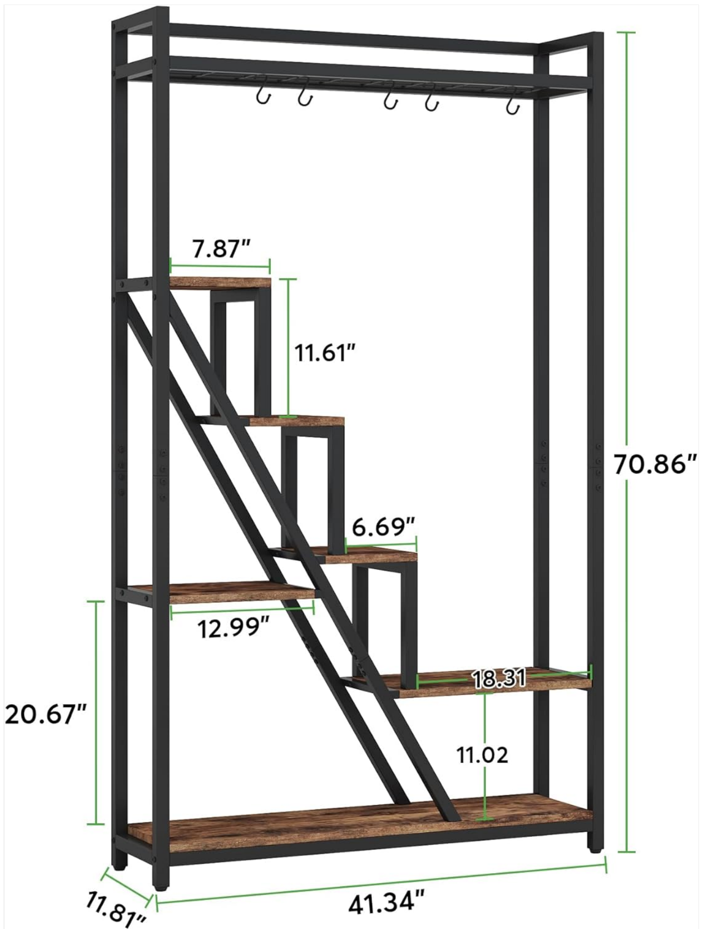
Figure 3.1: Detailed dimensions of the plant stand, showing its 70.86" height, 41.34" width, and 11.81" depth, along with individual shelf measurements.
