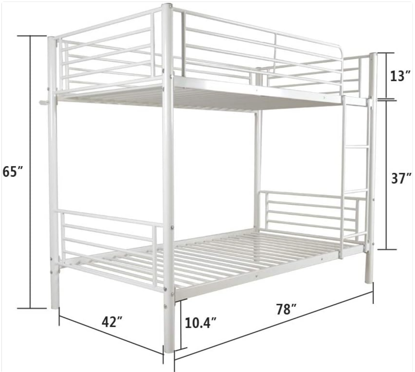
Figure 5: Dimensional diagram of the bunk bed, illustrating key measurements such as length, width, height, and guardrail height.
