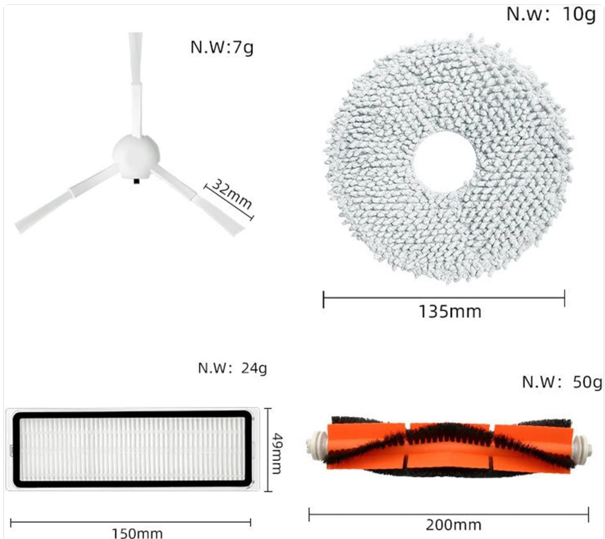
Image: Approximate dimensions and weights of individual components.
