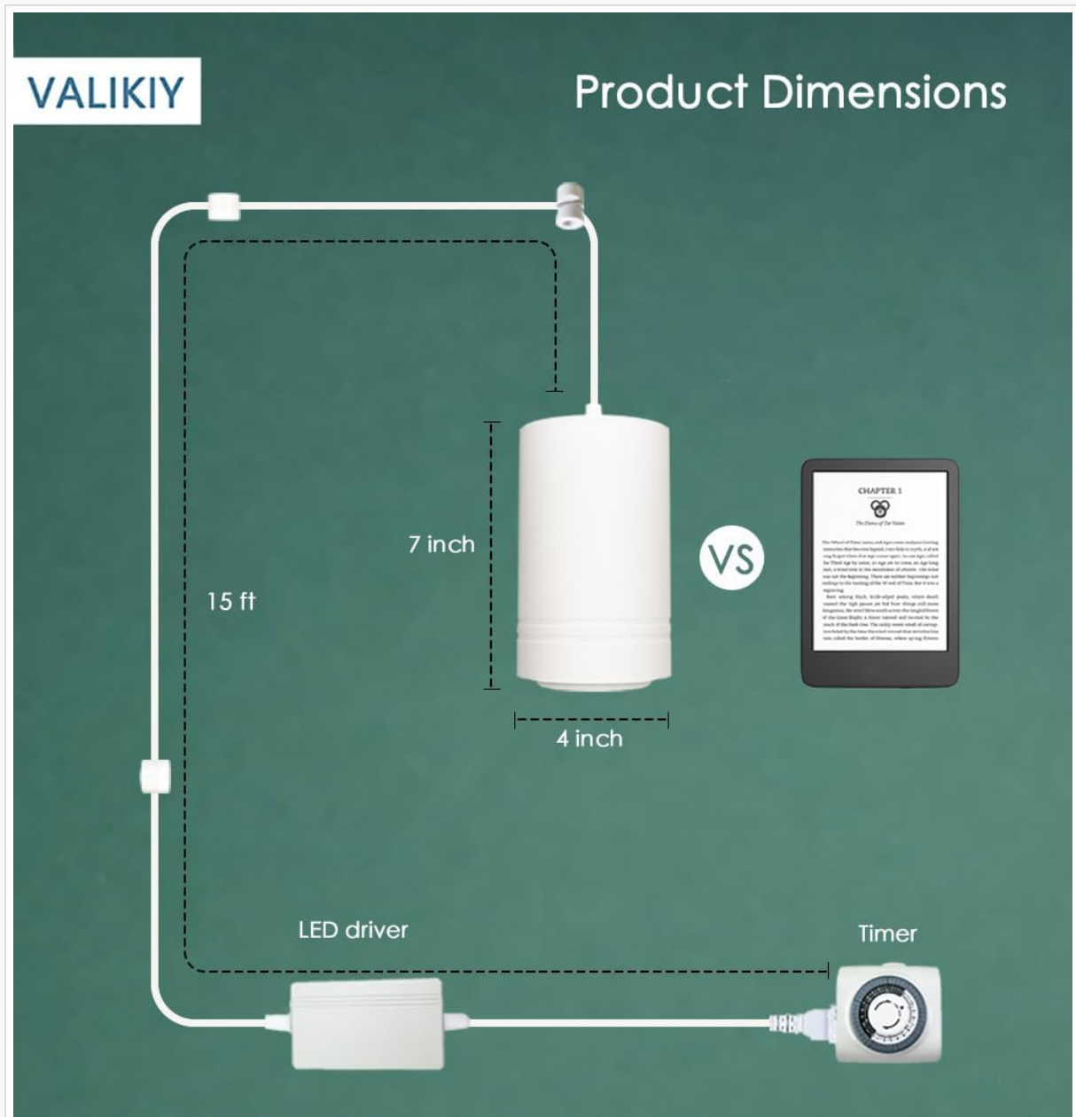
Image: Installation diagram for the VALIKIY Hanging Grow Light.
