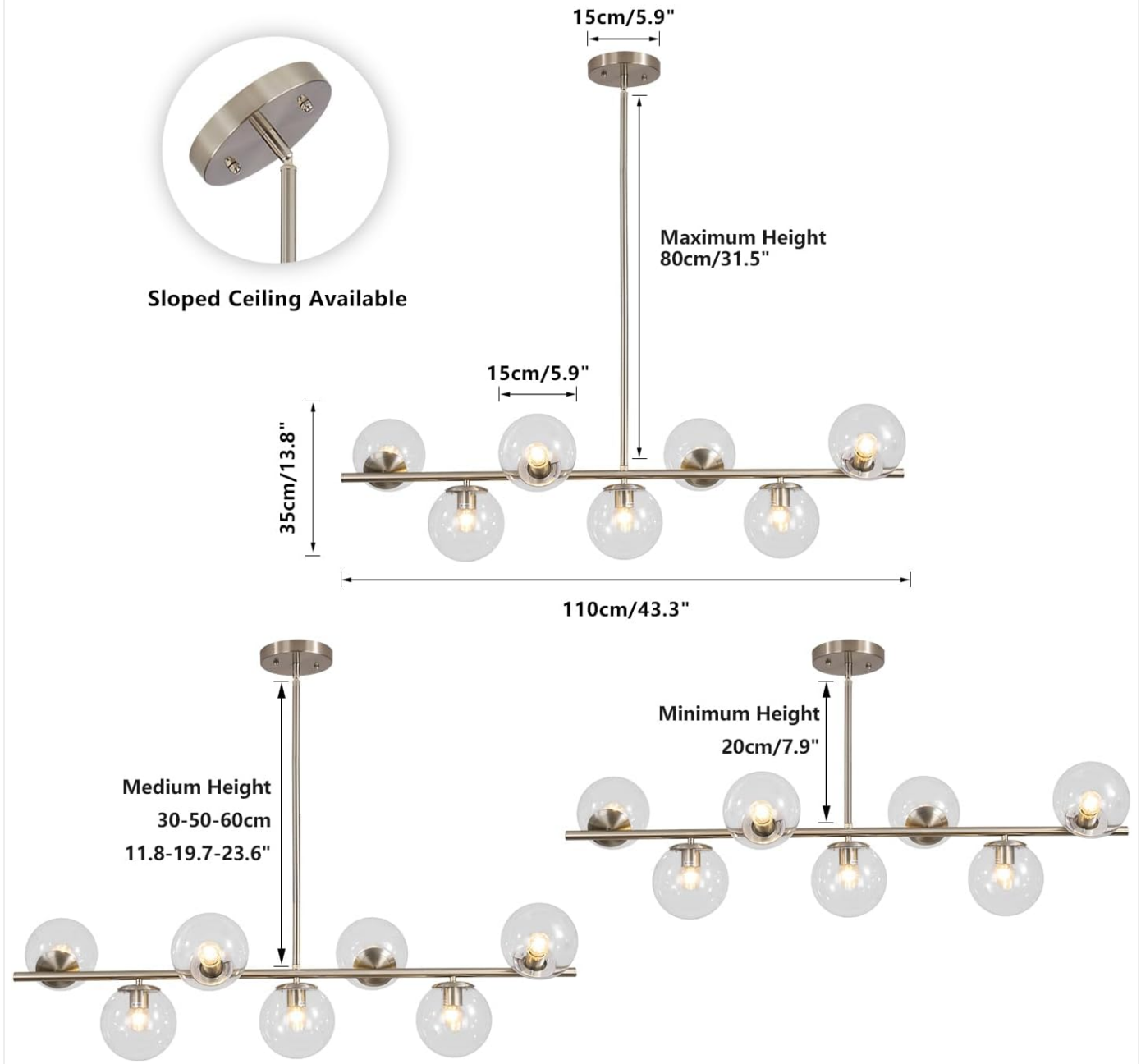
Figure 3.1: Product dimensions and illustration of sloped ceiling compatibility.
