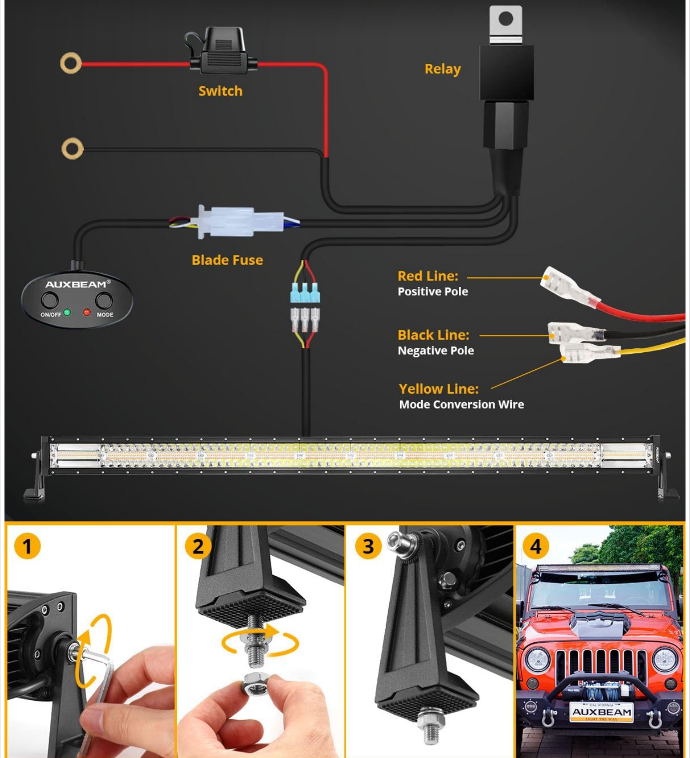
Image 4: Wiring diagram for the Auxbeam light bar.
