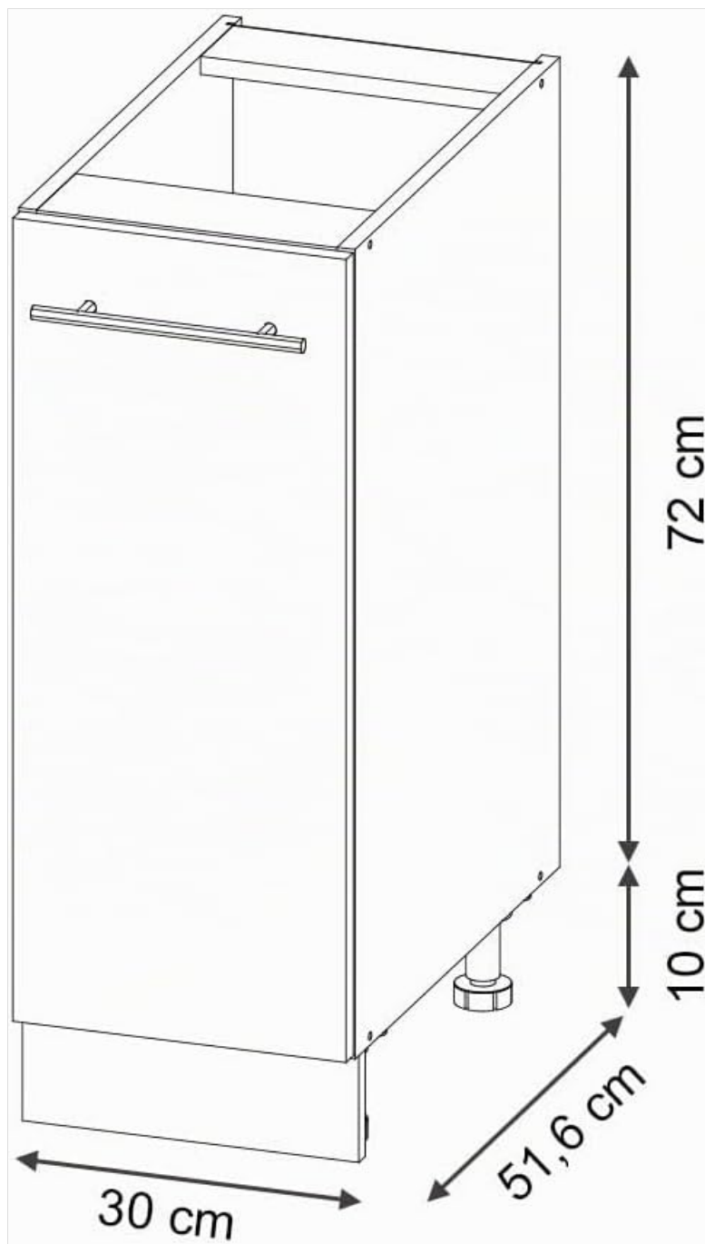
Figure 1: Cabinet Dimensions (Width: 30cm, Height: 82cm, Depth: 51.6cm)
