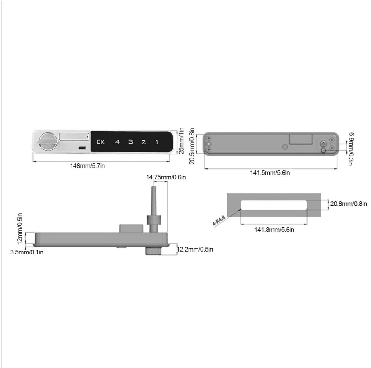
Image: Detailed dimensions of the lock unit, crucial for accurate installation.
