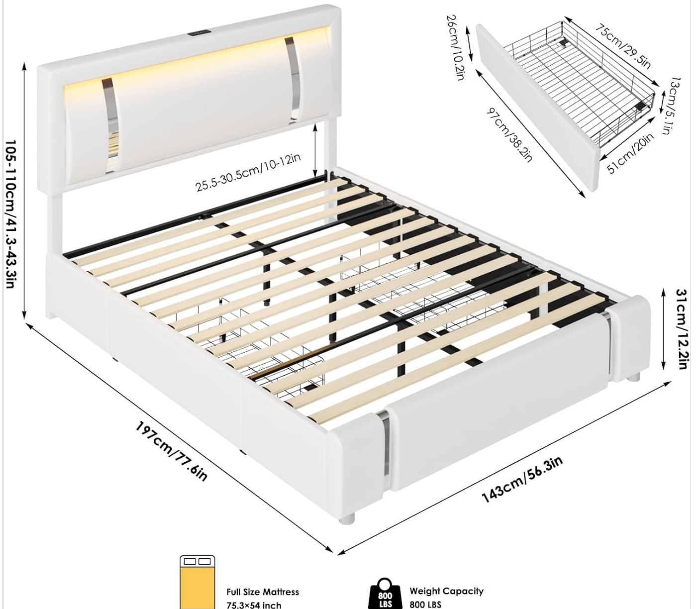
Figure 2.1: Overview of Keyluv KLV-UP-229 Full Size Bed Frame dimensions.
