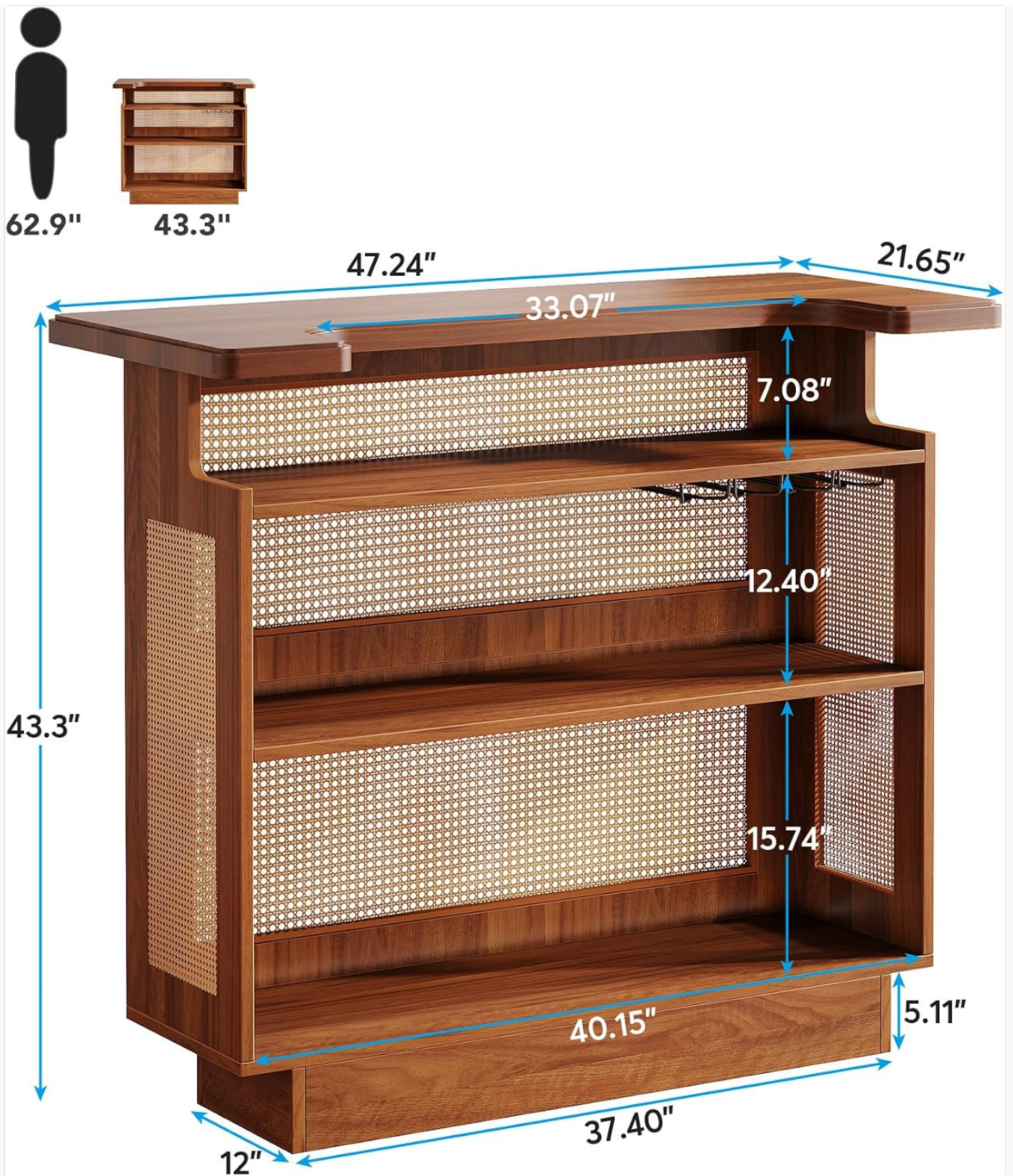
Image 4.1: Product dimensions for assembly reference.
