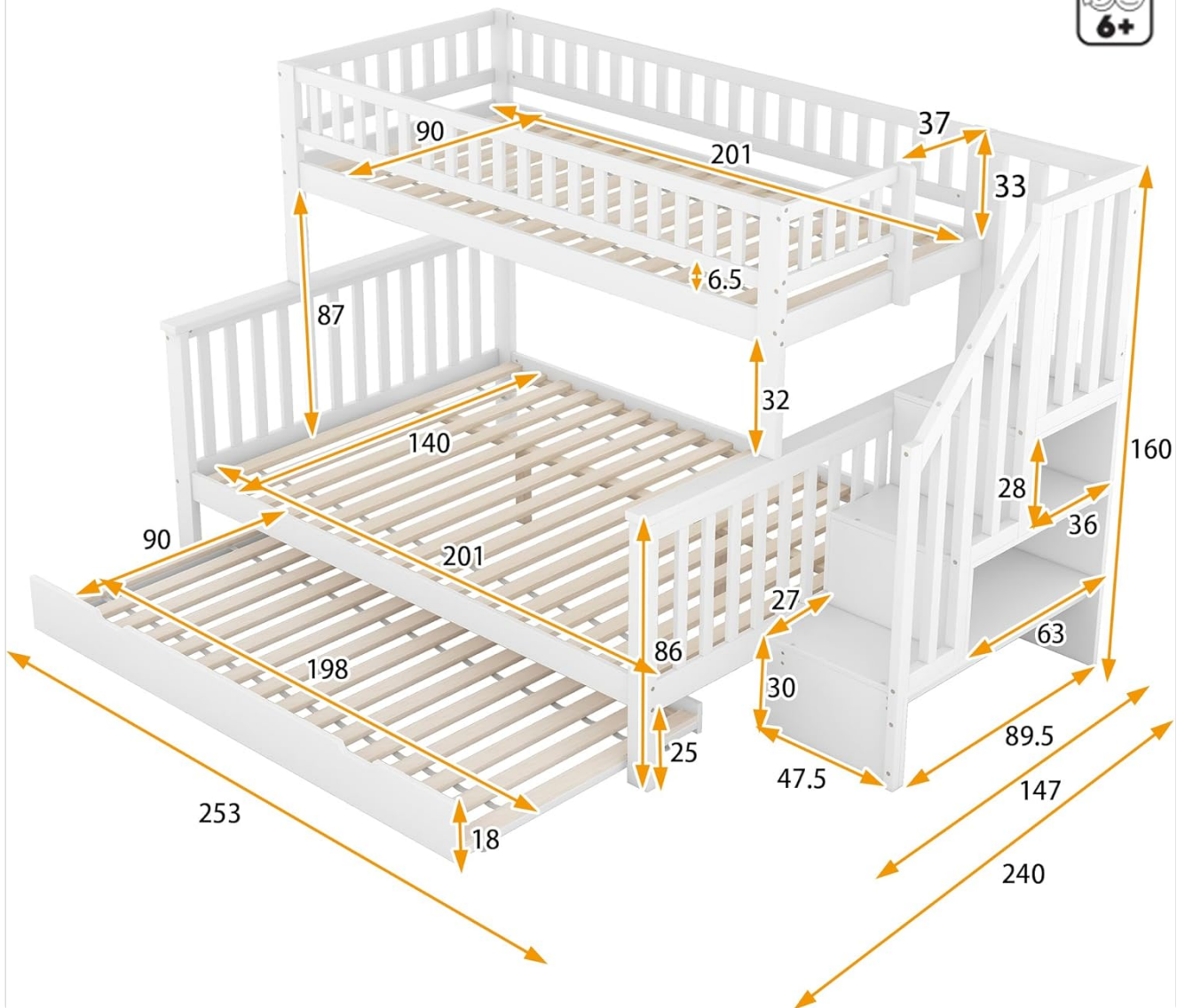
Figure 6: Detailed dimensions of the Moimhear Bunk Bed.
