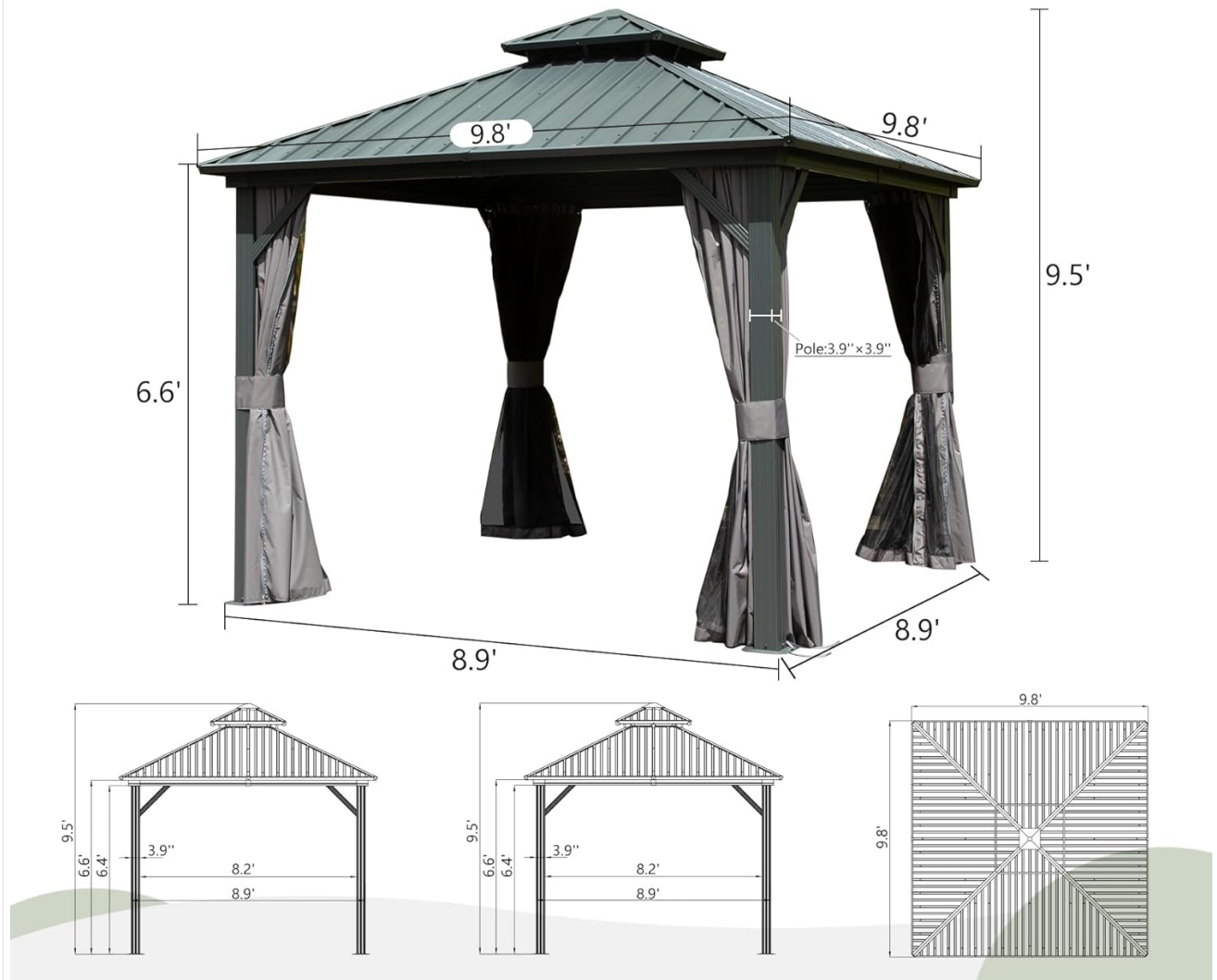
Figure 3.2: Dimensions of the 10' x 10' Hardtop Gazebo.
