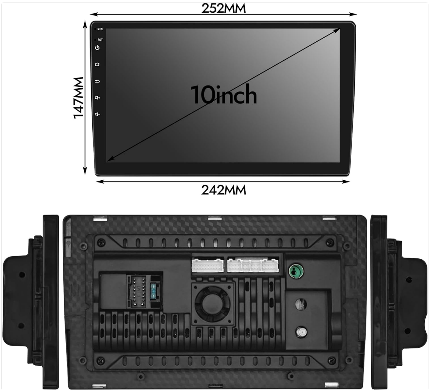
Image: Diagram showing the precise measurements of the 10-inch head unit, including width, height, and screen size.
