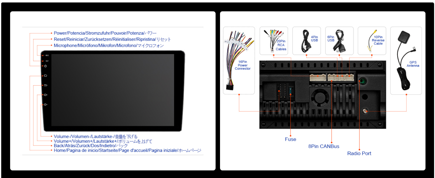
Image: Detailed wiring diagram illustrating the connections for the 16-pin power connector, RCA cables, USB ports, reverse cable, and GPS antenna on the back of the head unit.
