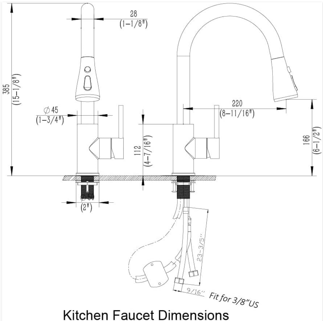
Image: Kitchen Faucet Dimensions for Model HV601.
