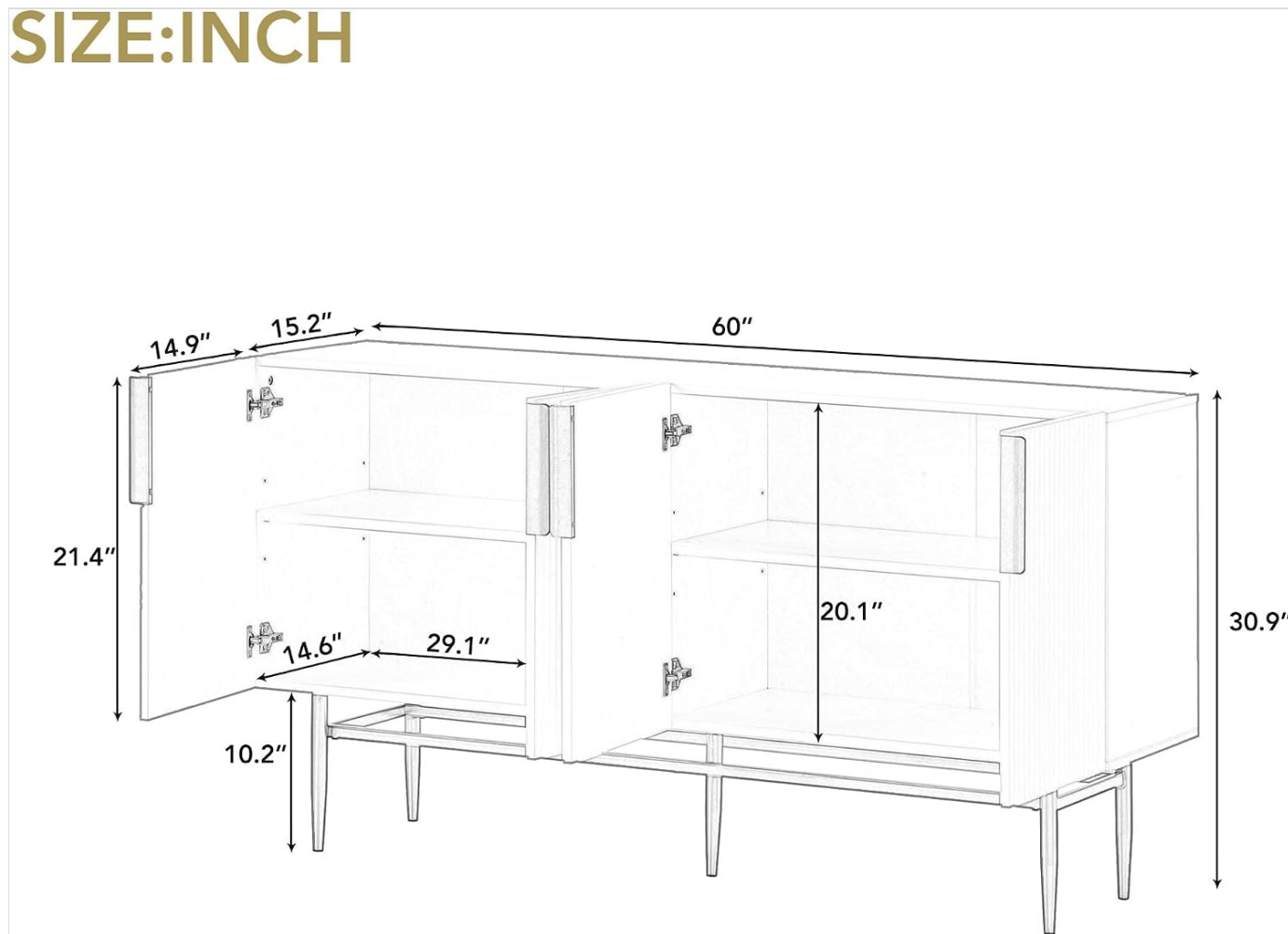
Figure 4.1: Cabinet dimensions. The overall dimensions are 60 inches wide, 15.2 inches deep, and 30.9 inches high. Internal shelf dimensions are also indicated.
