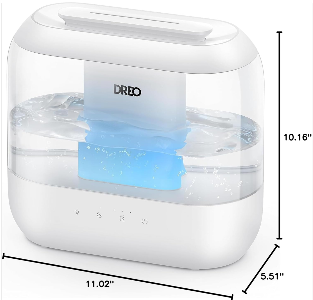
Figure 8: Detailed dimensions of the Dreco 4L Cool Mist Humidifier.
