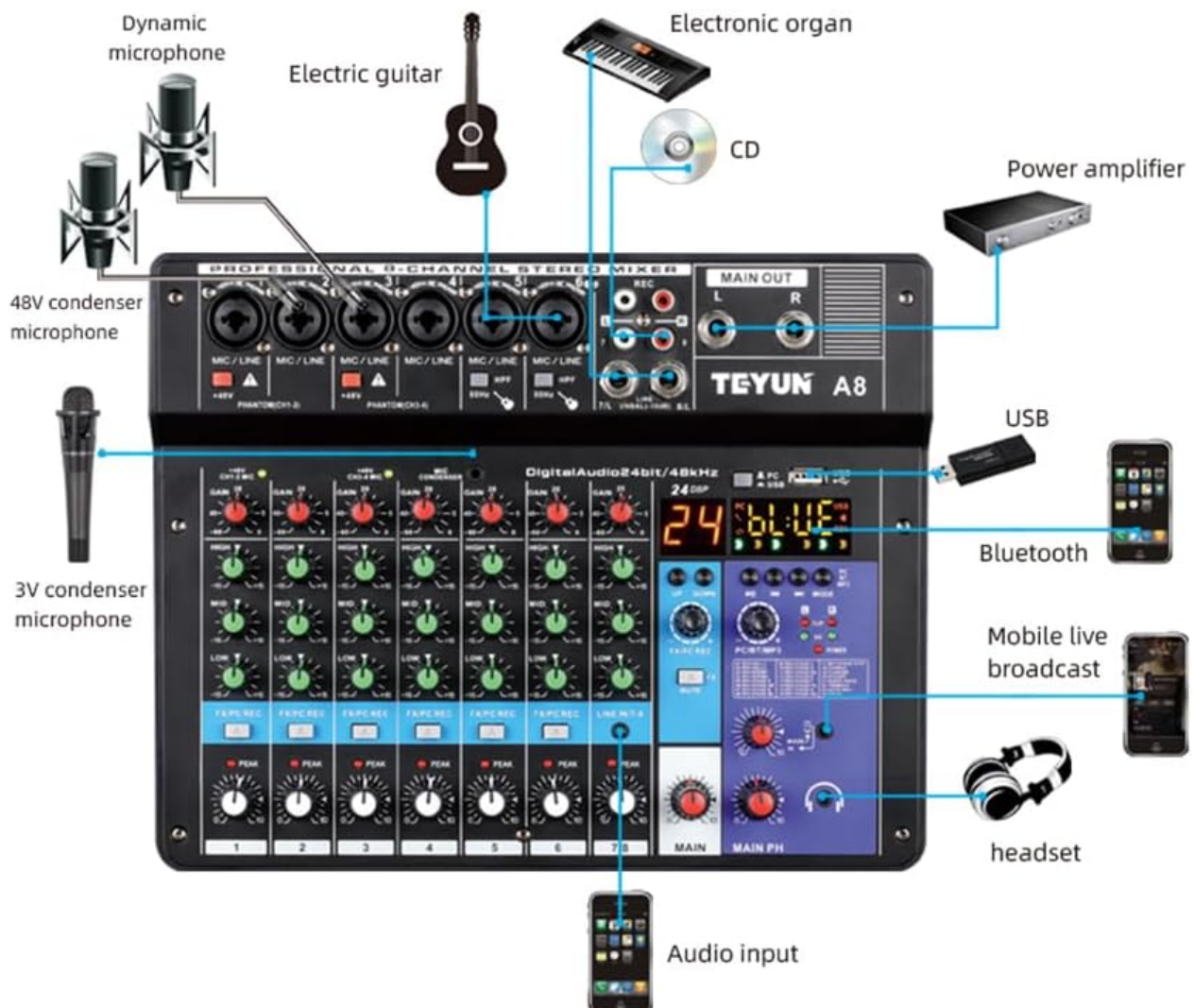
Figure 3: Detailed connection diagram for the mixer.
