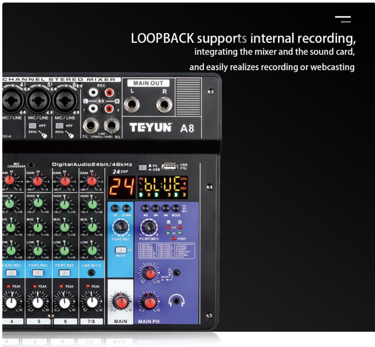
Figure 5: Digital display and main control section, featuring loopback recording.
