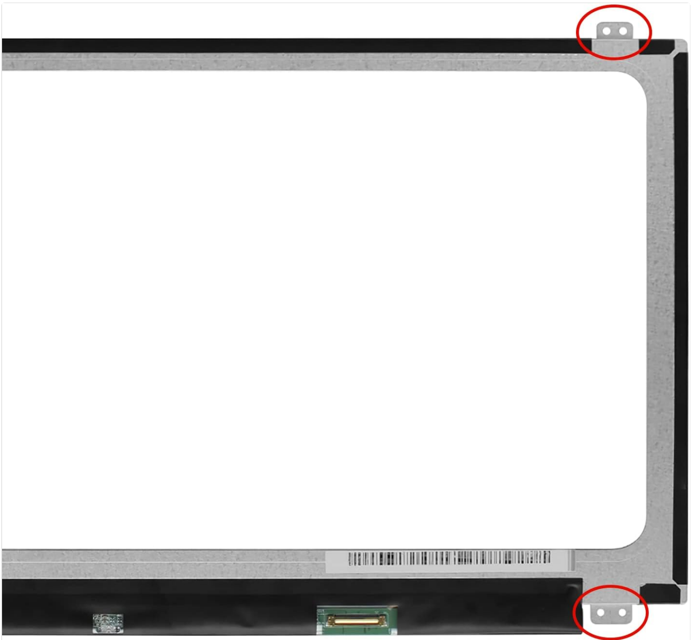
Figure 4.2: Example of mounting tabs on the LCD panel, typically located at the top and bottom corners, used to secure the screen within the laptop lid.
