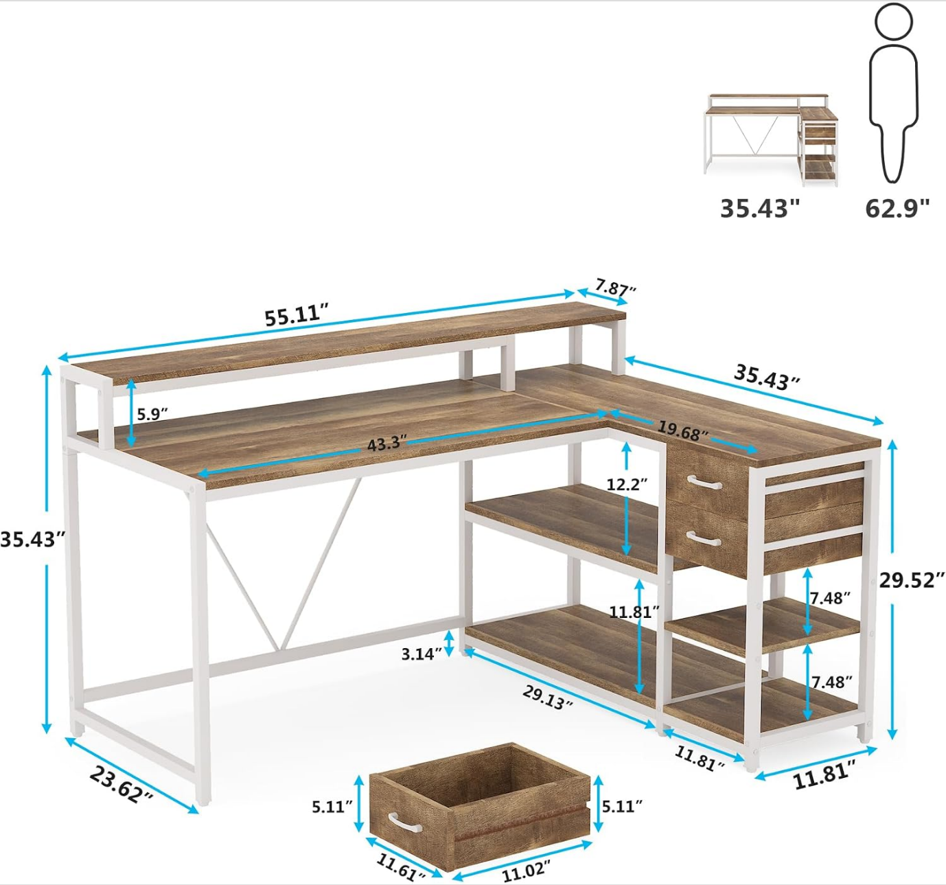
Image: A technical drawing illustrating the overall dimensions and key measurements of the L-shaped desk.
