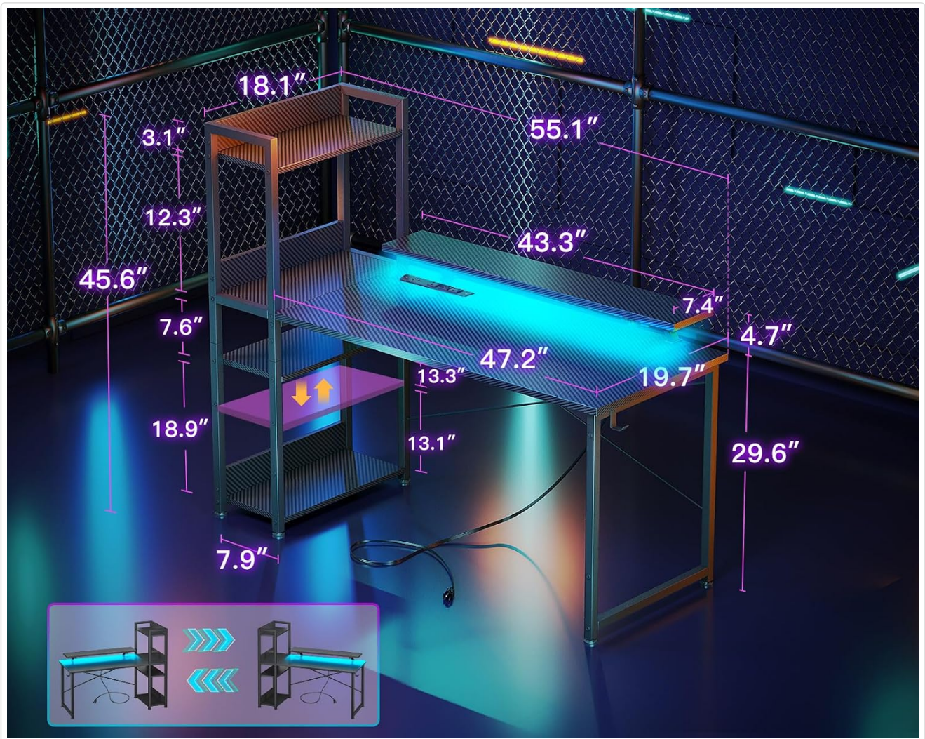
Image: Detailed dimensions of the ODK 55 Inch Gaming Desk, including the main tabletop, monitor stand, and reversible storage shelves.
