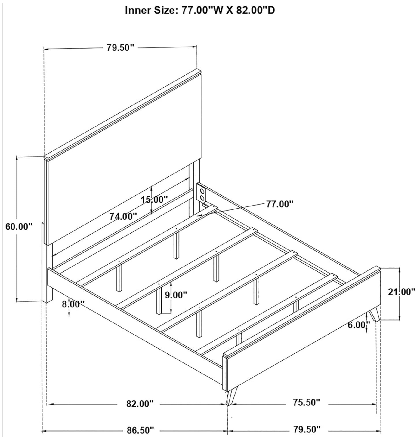
Figure 3: Dimensional drawing of the bed frame, providing key measurements for length, width, and height, including the headboard and footboard dimensions. Inner dimensions for mattress placement are also shown.
