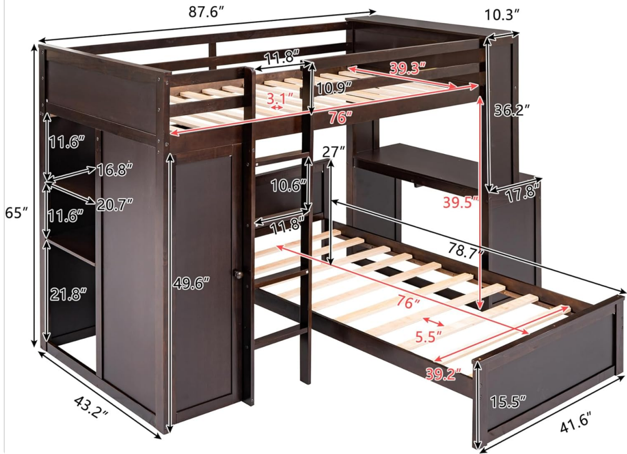
Figure 5: Detailed dimension diagram of the TRIPLE TREE Twin Size Loft Bed, showing length, width, and height measurements for all sections.
