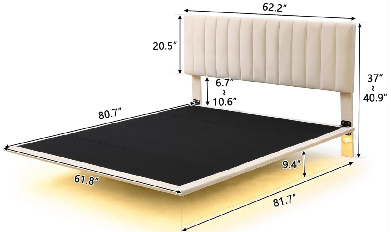
Image: Overview of the bed frame components with key dimensions.
