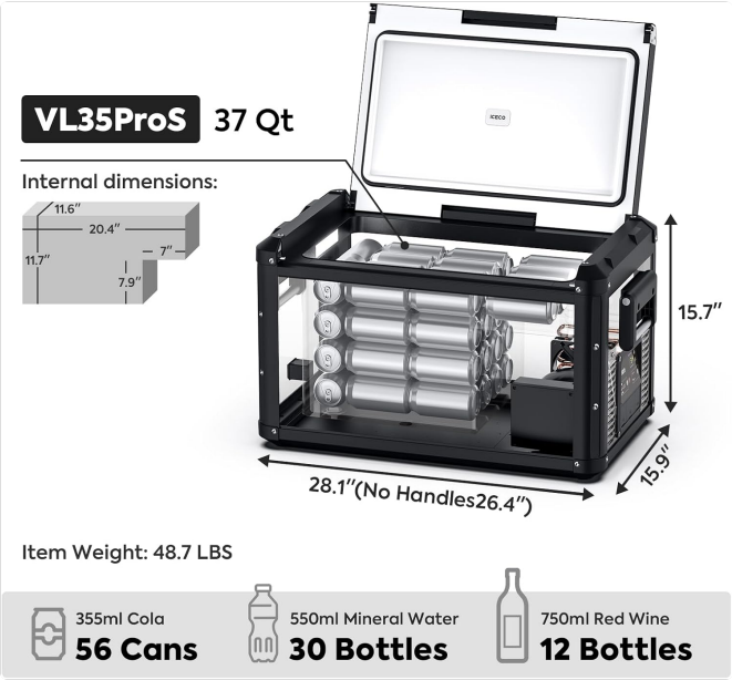
Figure 3.2: Dimensions and Capacity Overview
