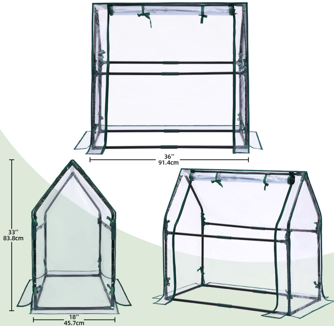
Figure 7: Greenhouse dimensions.
