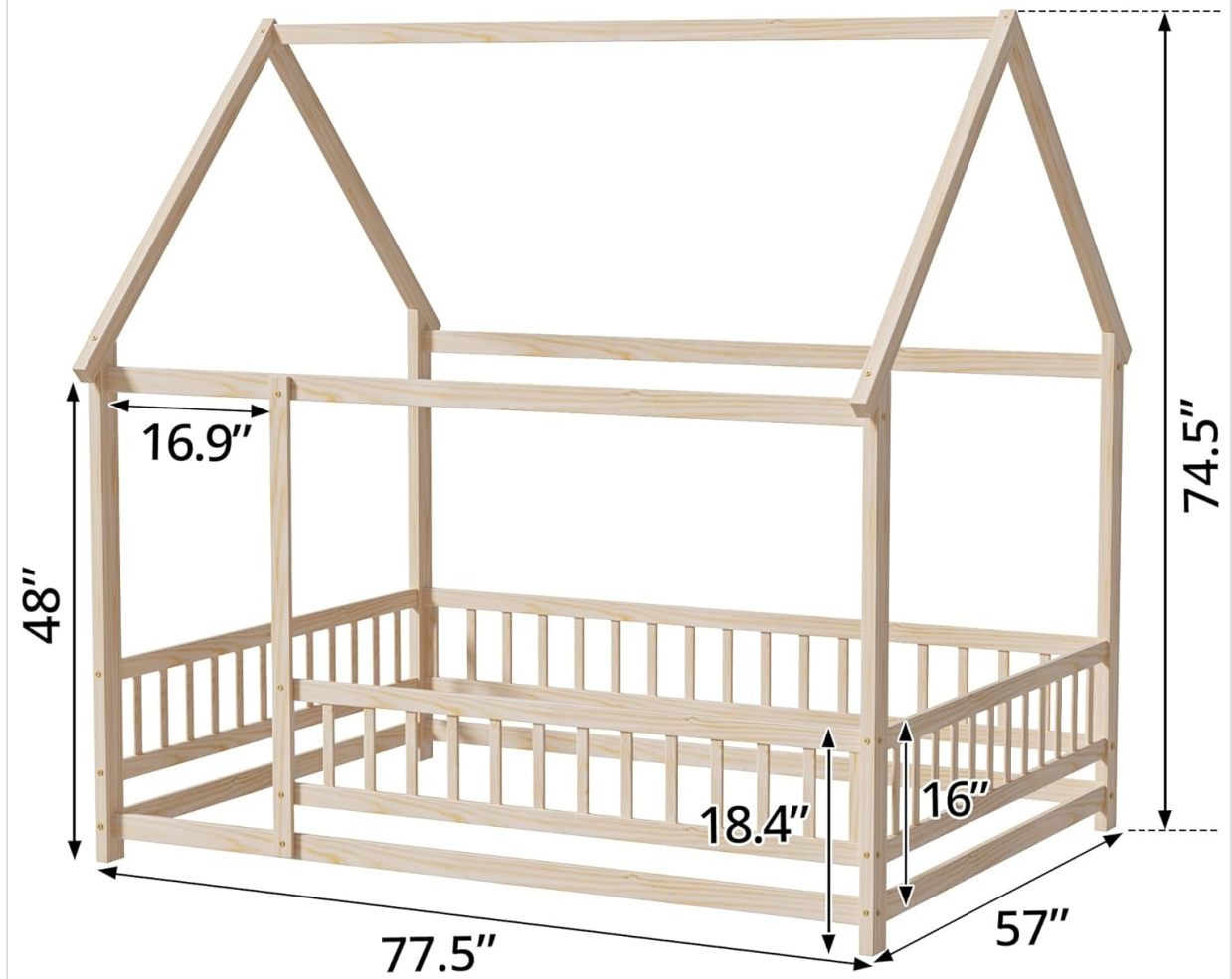
Diagram illustrating the dimensions of the LLS Full Size House Bed with Fence.
