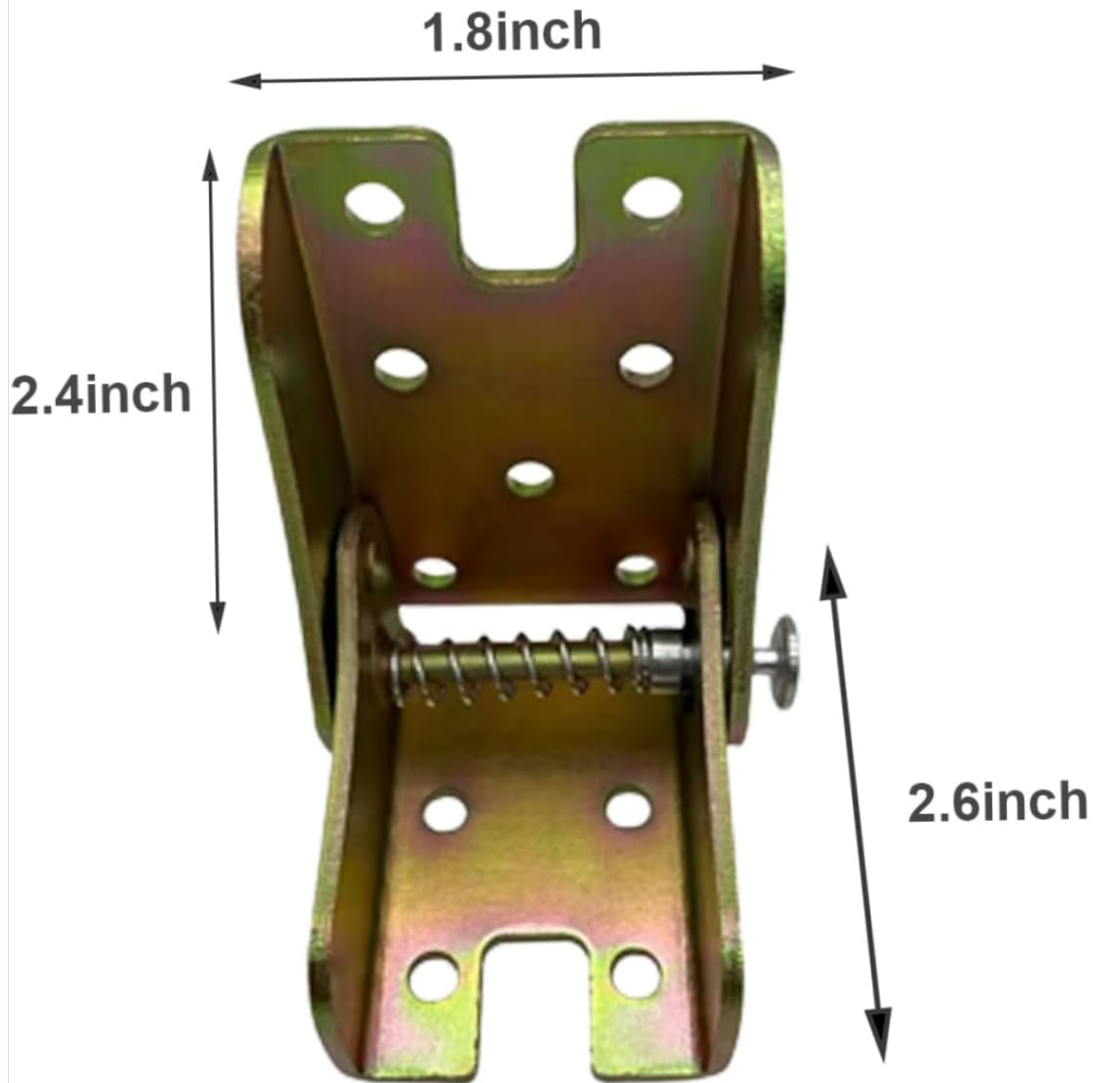
Image 6.1: Product dimensions for the SENRN 90 Degree Self-Locking Folding Hinge.
