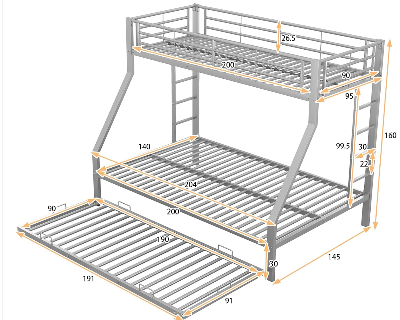
Image: Technical diagram showing the dimensions of the Moimhear Metal Bunk Bed in centimeters. Key measurements include overall length (204 cm), width (145 cm), height (160 cm), and individual bunk and trundle dimensions.
