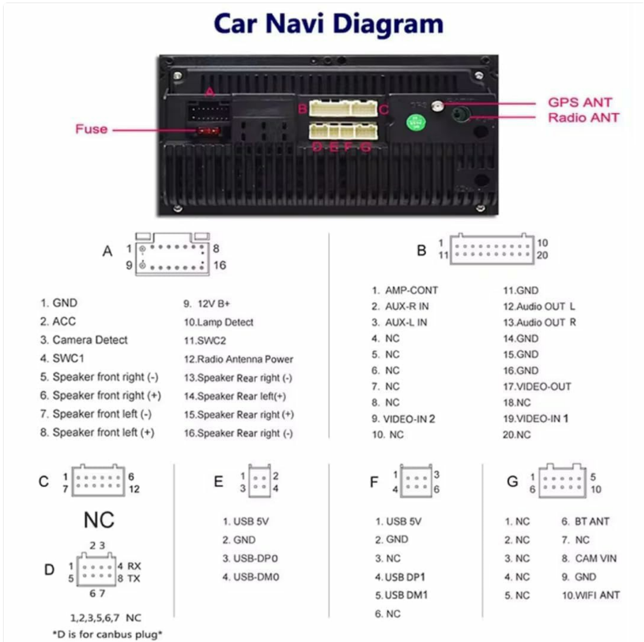
Figure 4.2: Car Navi Diagram. This diagram details the various connection ports on the rear of the unit, including power, speaker outputs, auxiliary inputs, video inputs/outputs, USB ports, and antenna connections for GPS, Radio, Bluetooth, and WiFi.
