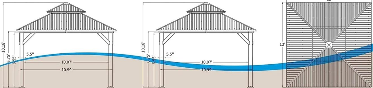
Figure 5: Gazebo dimensions.
