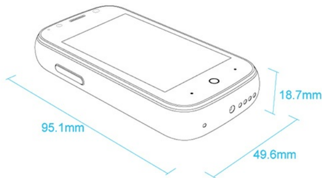
Figure 8.1: Product Dimensions.
