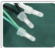
Figure 4.3: Visual guide for the electrical wiring connection process, ensuring wires are secured and not exposed to the cooking area.
