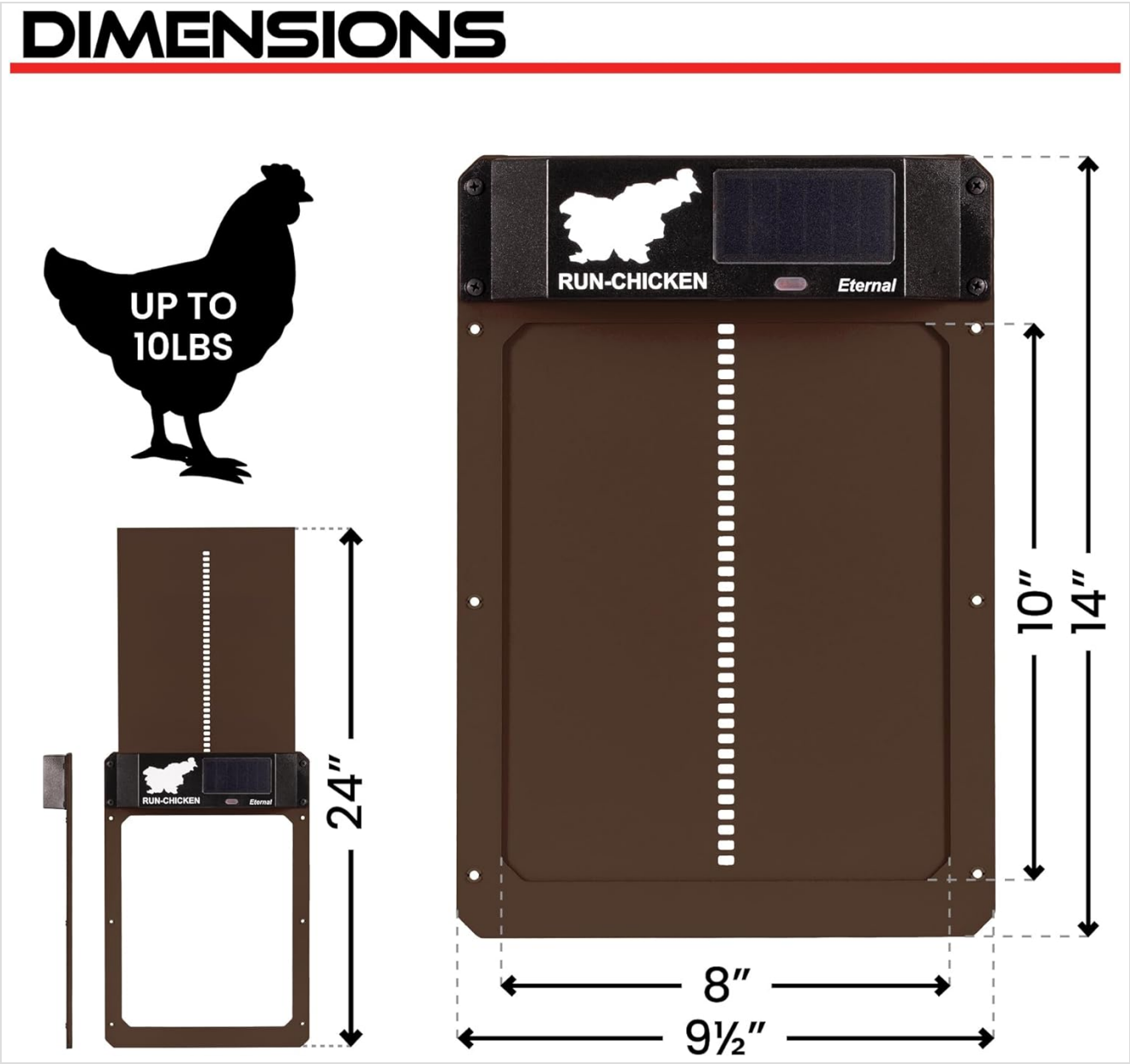
Image 10.1: Dimensions of the RUN-CHICKEN Eternal door.
