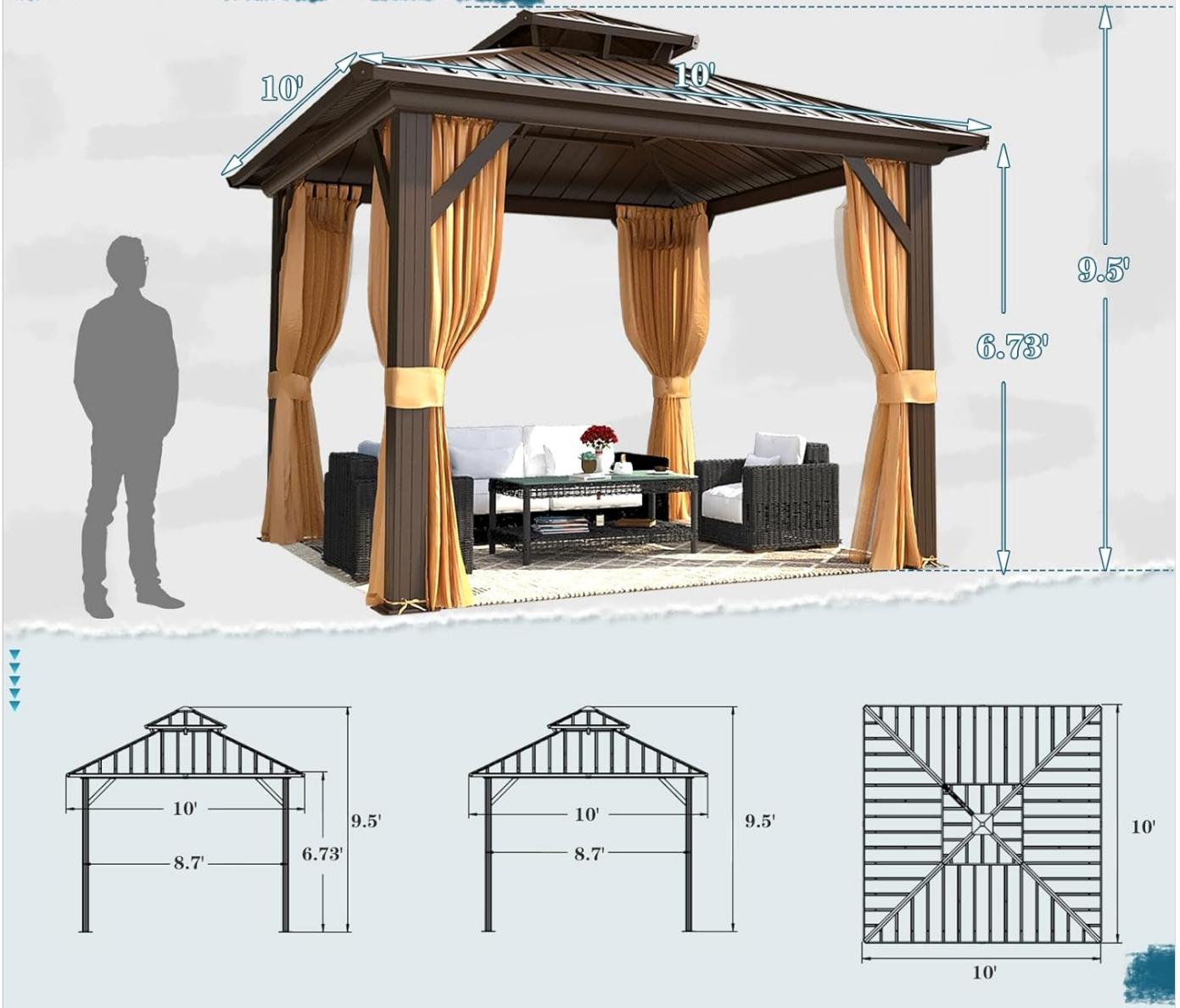
Figure 6: Detailed dimensions and size description for the 10'x10' gazebo.
