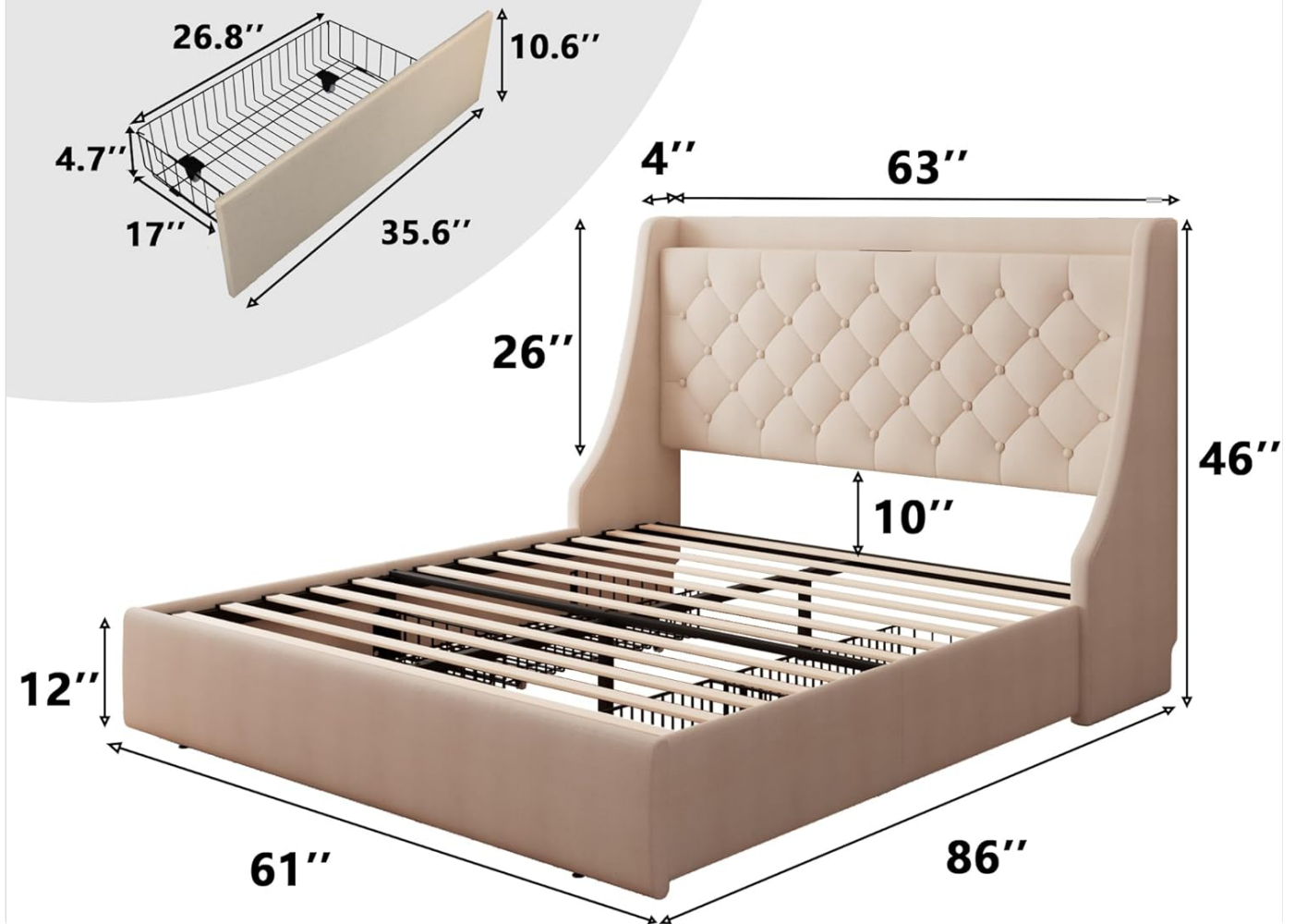
Figure 10: Queen Size Bed Frame Dimensions.
