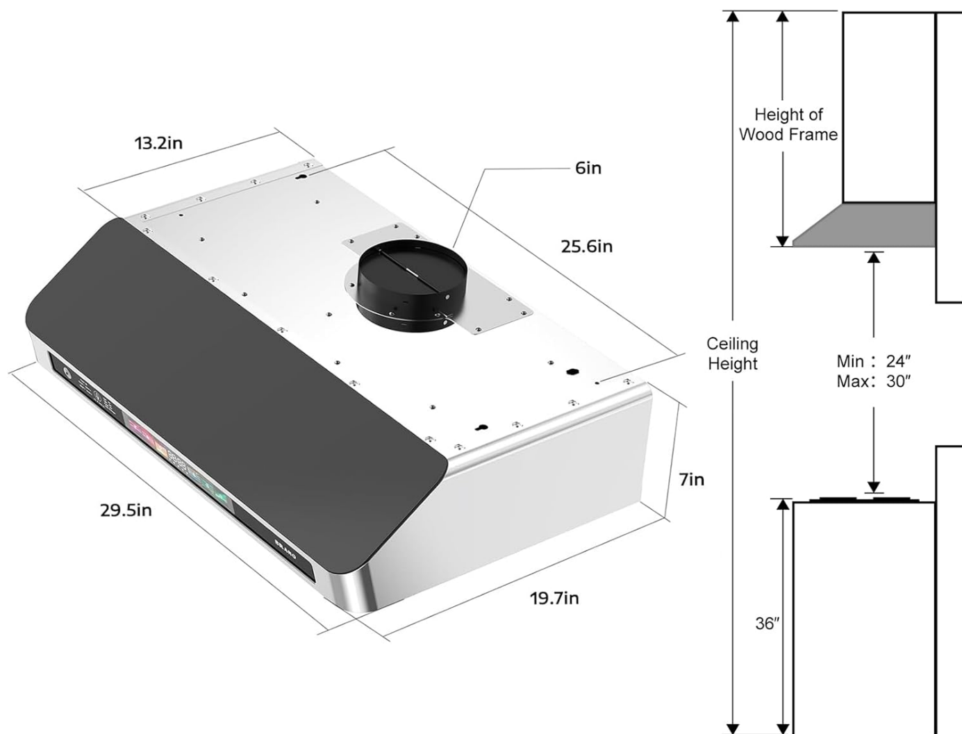
Figure 1: Product Dimensions and Installation Clearances. The hood measures 29.5 inches wide, 19.7 inches deep, and 7 inches high. Recommended installation height from cooking surface is between 24 and 30 inches.
