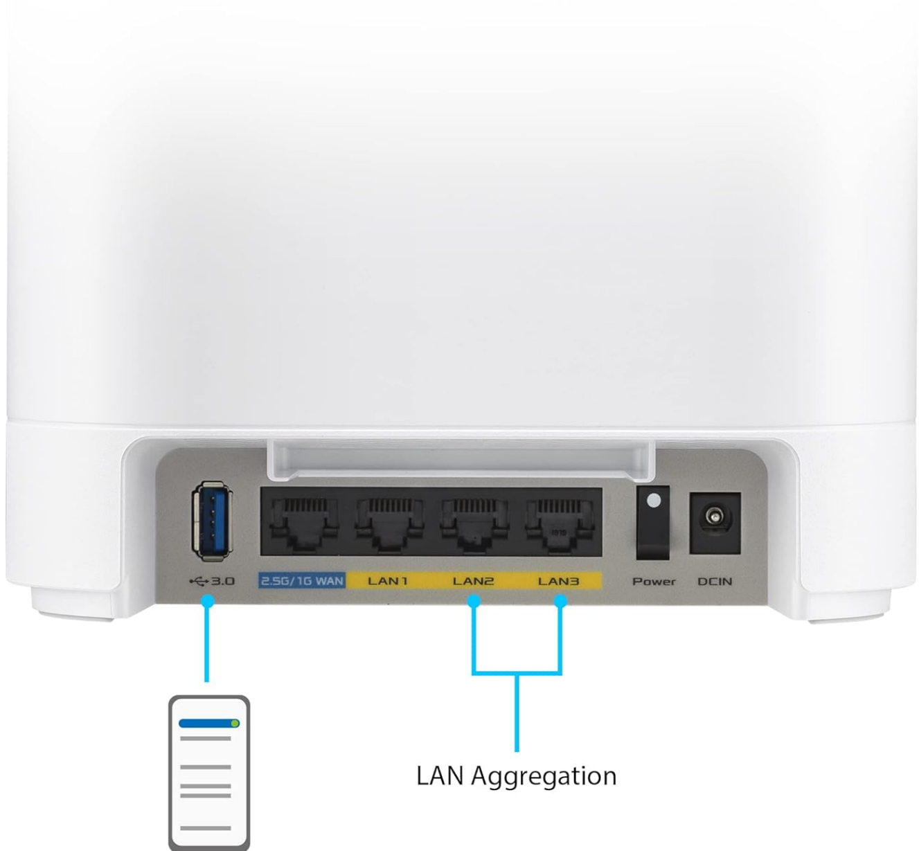
Image: The rear view of the ASUS ExpertWiFi EBM68, highlighting its various ports including USB 3.0, 2.5G/1G WAN, multiple LAN ports, and power input, demonstrating its versatile connectivity.
