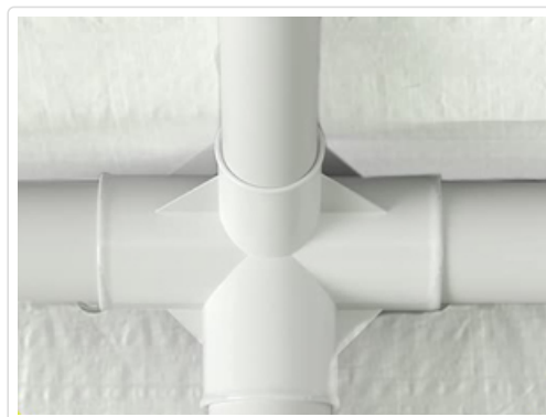
Figure 4.2: Detail of a double reinforced connector, ensuring frame stability.
