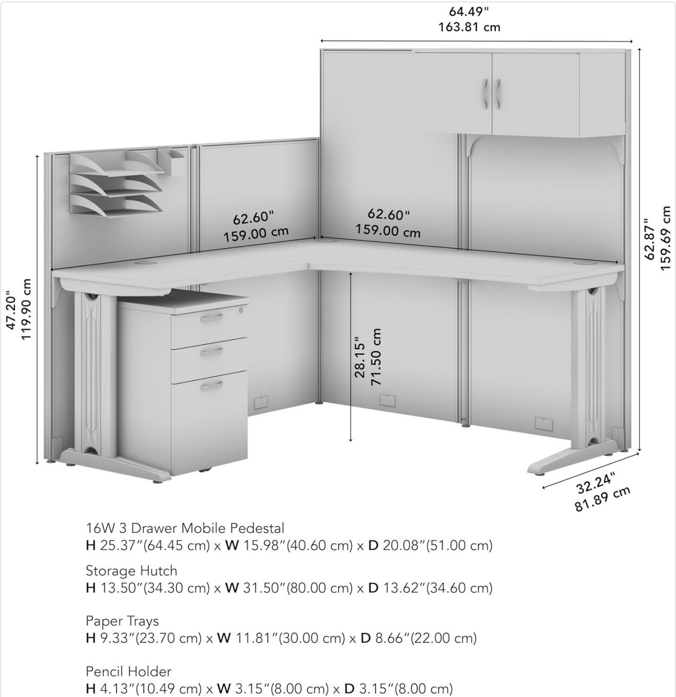
Figure 4.1: Dimensional overview of the L-shaped cubicle desk, mobile pedestal, storage hutch, paper trays, and pencil holder.
